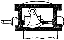
RELIEF VALVES.
